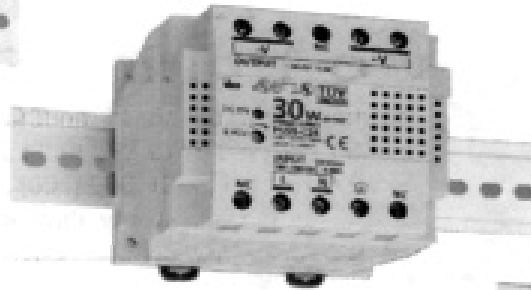
30W Part No. PS5R-C12 (output: 12VDC/2.5A)
