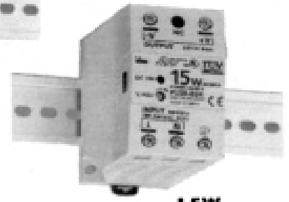
15W Part No. PS5R-A12 (output: 12VDC/0.6A)
