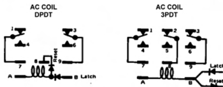
WIRING DIAGRAMS FOR 166ML SERIES
