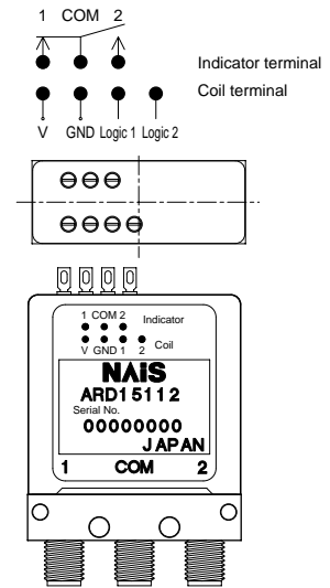
Latching with TTL driver (with self cut-off function)
