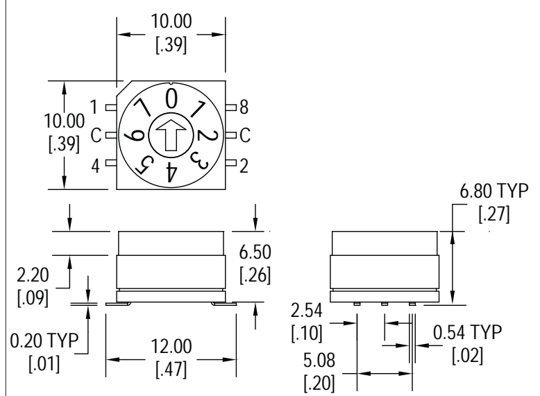
G Terminals
