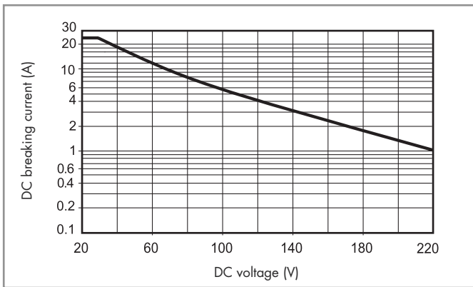
H 22 - Maximum DC1 breaking capacity - Type 22.32 / 22.34
