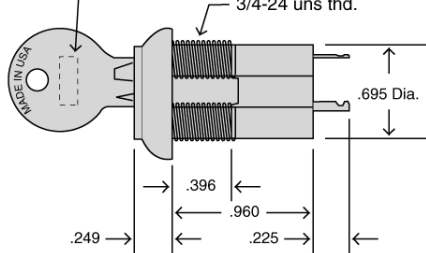
PC Mounting
