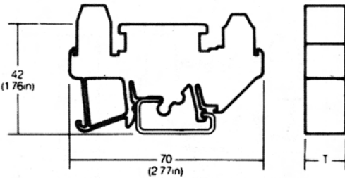
"H" dimension 5mm less on TS 35 x 7.5 rail
