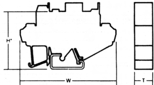
"H" dimension 5mm less on TS 35 x 7.5 rail * Height shown to top of socket—add I/O module for overall height.
