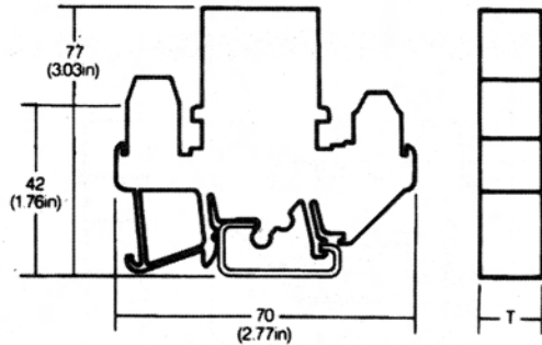
"H" dimension 5mm less on TS 35 x 7.5 rail
