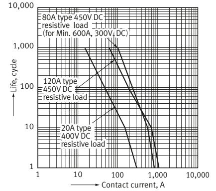
4. Switching and cut-off life curve (Forward direction)
