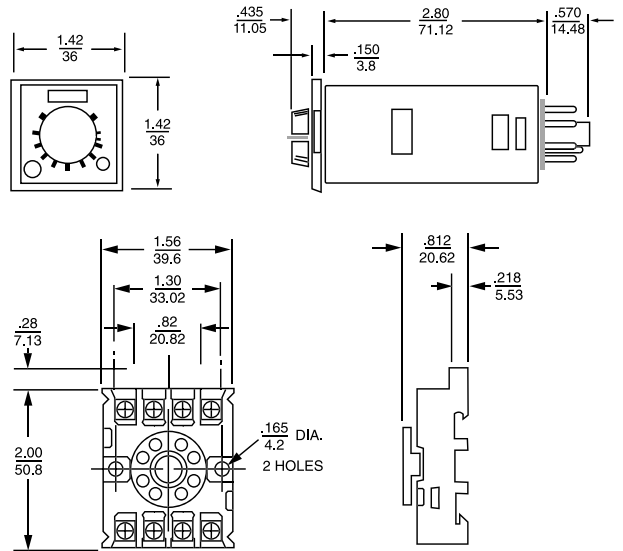
8 PIN OPTIONAL OCTAL SOCKET NO. 00008258500
