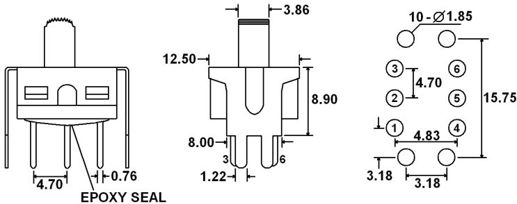
S20 = PC Pins with Support Bracket, Double Pole
