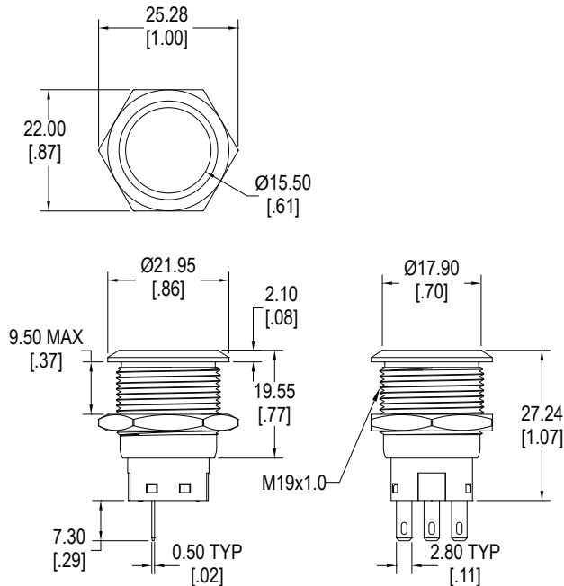
A - Flush Actuator, Non-Illuminated
