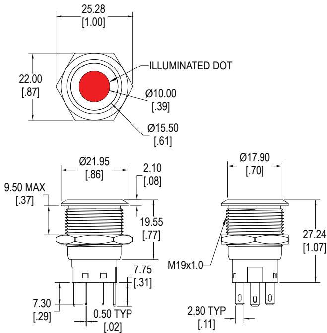
C - Flush Actuator, Dot Illuminated
