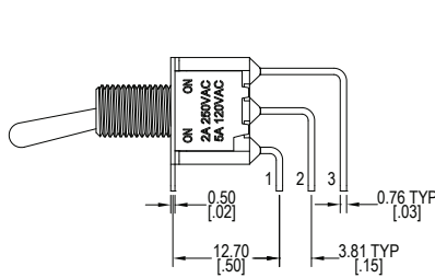
V (VS - Snap-in) = Vertical mount, right angle PC pins, single pole
