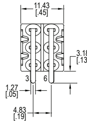
V (VS - Snap-in) = Vertical mount, right angle PC pins, double pole
