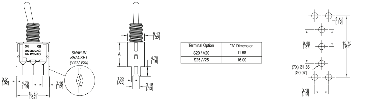
S20/S25 (V20/V25 - Snap-in) = PC pins with support bracket, single pole
