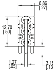
V (VS - Snap-in) = Vertical mount, right angle PC pins, single pole
