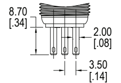
Quick Connect
