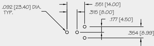
Fig. 1 PC BOARD LAYOUT
