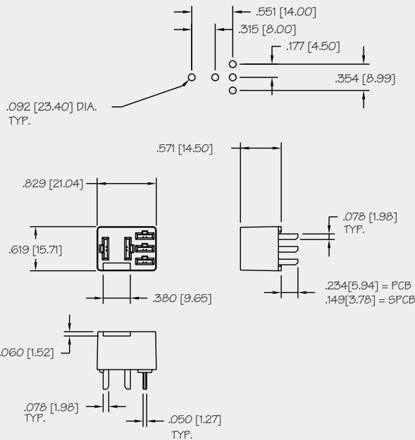
Fig. 2 PC BOARD LAYOUT
