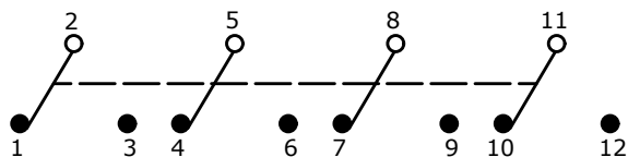
CIRCUIT: 4PDT
