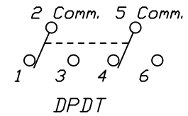
CONTACT CONFIGURATION
