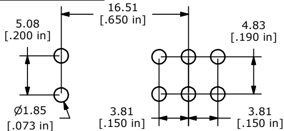
PCB MOUNTING
