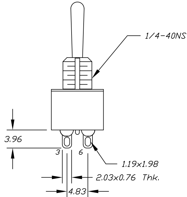
CIRCUIT: DPDT CONTACT CONFIGURATION
