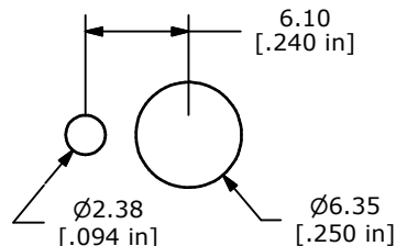
With Standard Locking Ring
