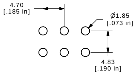
P.C. MOUNTING
