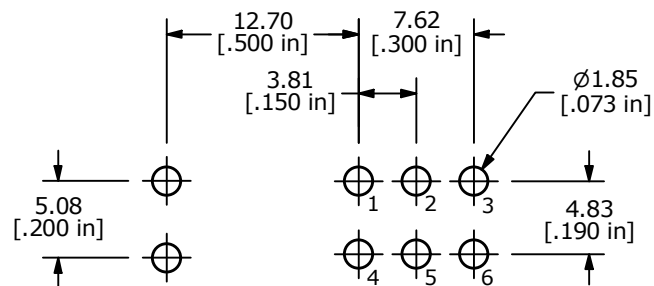
P.C. MOUNTING
