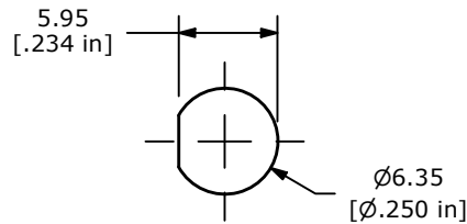
RECOMMENDED PANEL MOUNTING
