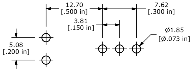
PCB LAYOUT
