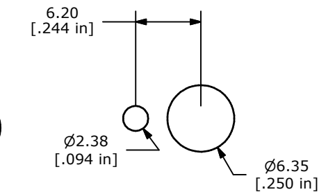
PANEL MOUNTING
