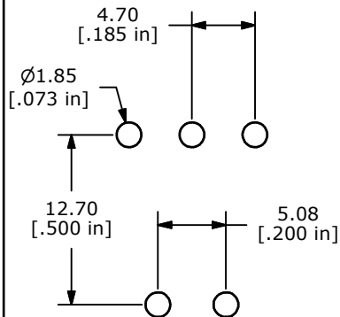
P.C. MOUNTING
