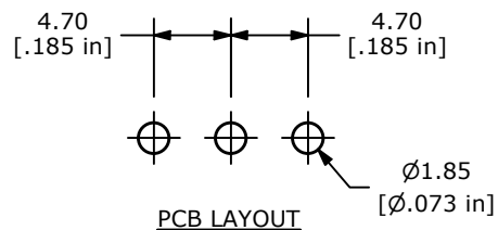
PCB LAYOUT
