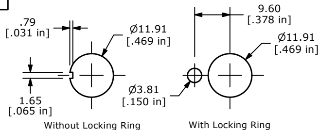
PANEL MOUNTING
