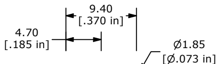
RECOMMENDED PANEL MOUNTING
