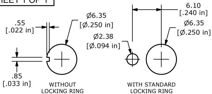
RECOMMENDED PANEL MOUNTING
