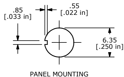
PANEL MOUNTING
