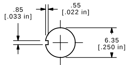
PANEL MOUNTING
