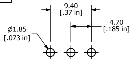
RECOMMENDED PC MOUNTING
