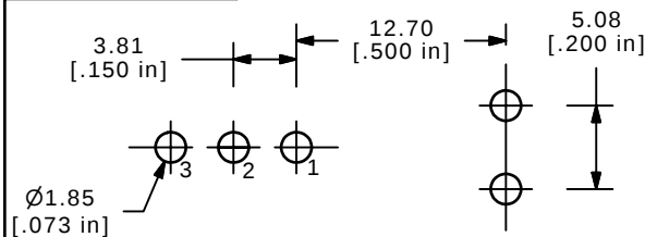
P.C. MOUNTING
