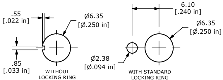
RECOMMENDED PANEL MOUNTING
