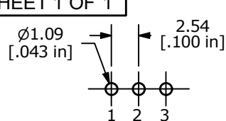
PCB MOUNTING
