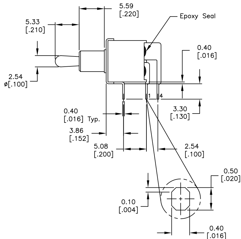
CIRCUIT: DPDT CONTACT CONFIGURATION
