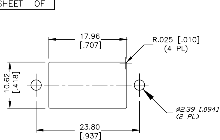
RECOMMENDED PANEL MOUNTING
