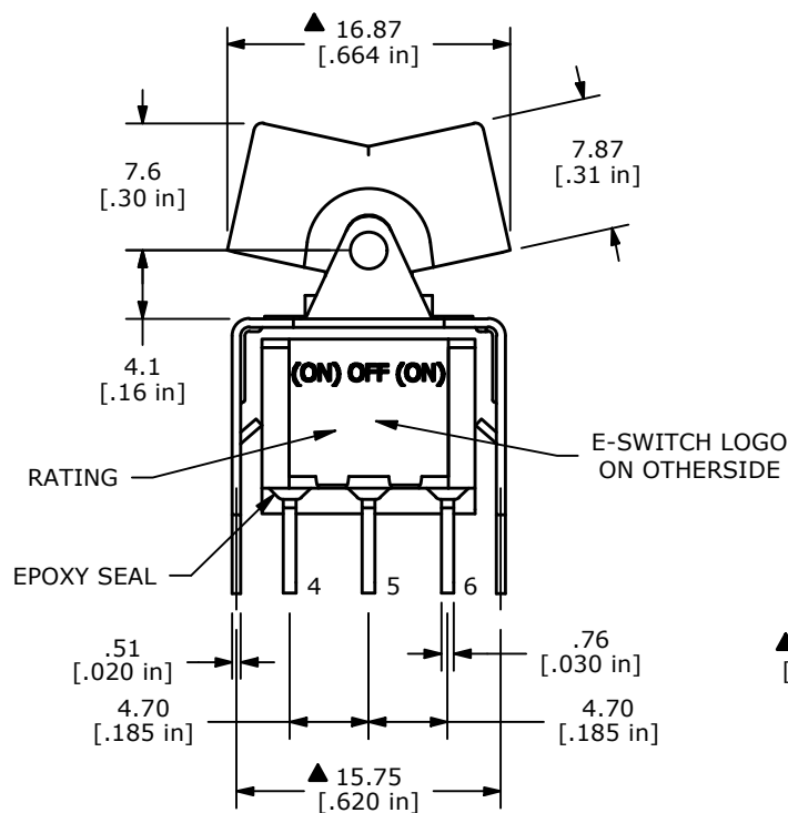
CIRCUIT: DPDT
