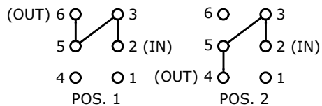
DPDT 3 WAY CIRCUIT
