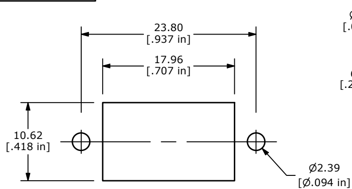
RECOMMENDED PANEL MOUNTING
