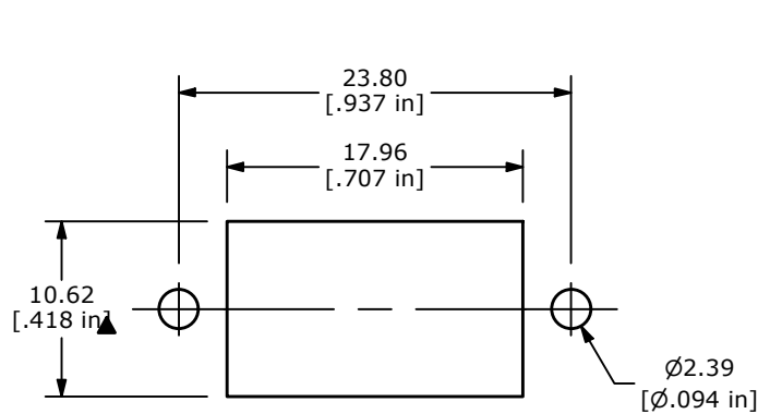
RECOMMENDED PANEL MOUNTING
