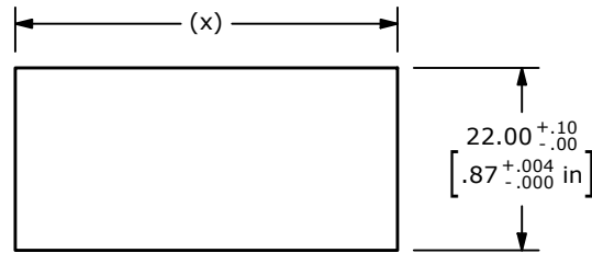
PANEL CUTOUT
