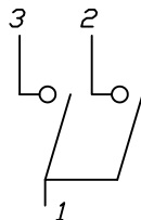
CIRCUIT: DPST CONTACT CONFIGURATION
