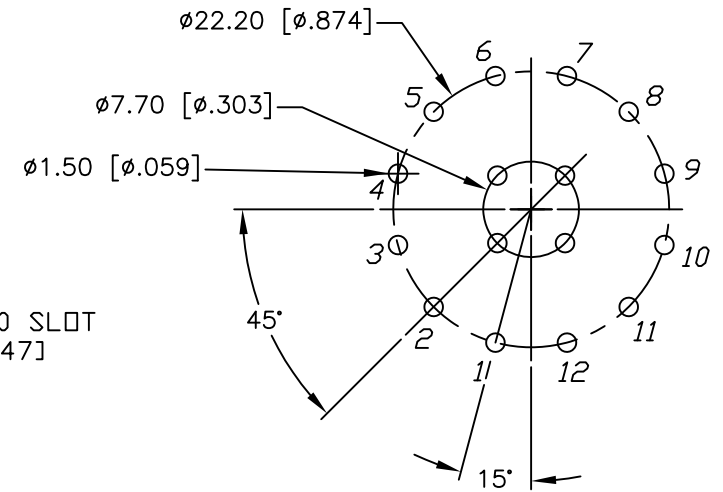
P.C.B. MOUNTING HOLES
