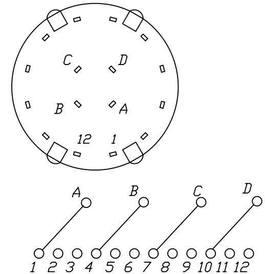
CONTACT CONFIGURATION
