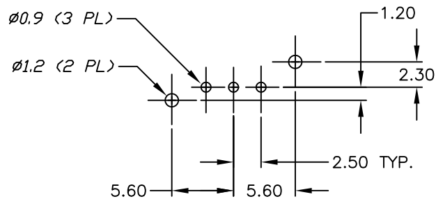
RECOMMENDED P.C.B. HOLES
