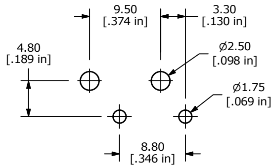
P.C. MOUNTING
