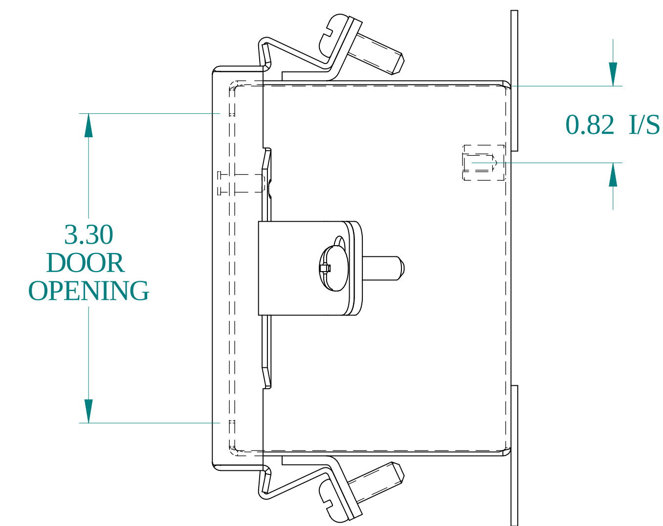
SIDE VIEW
