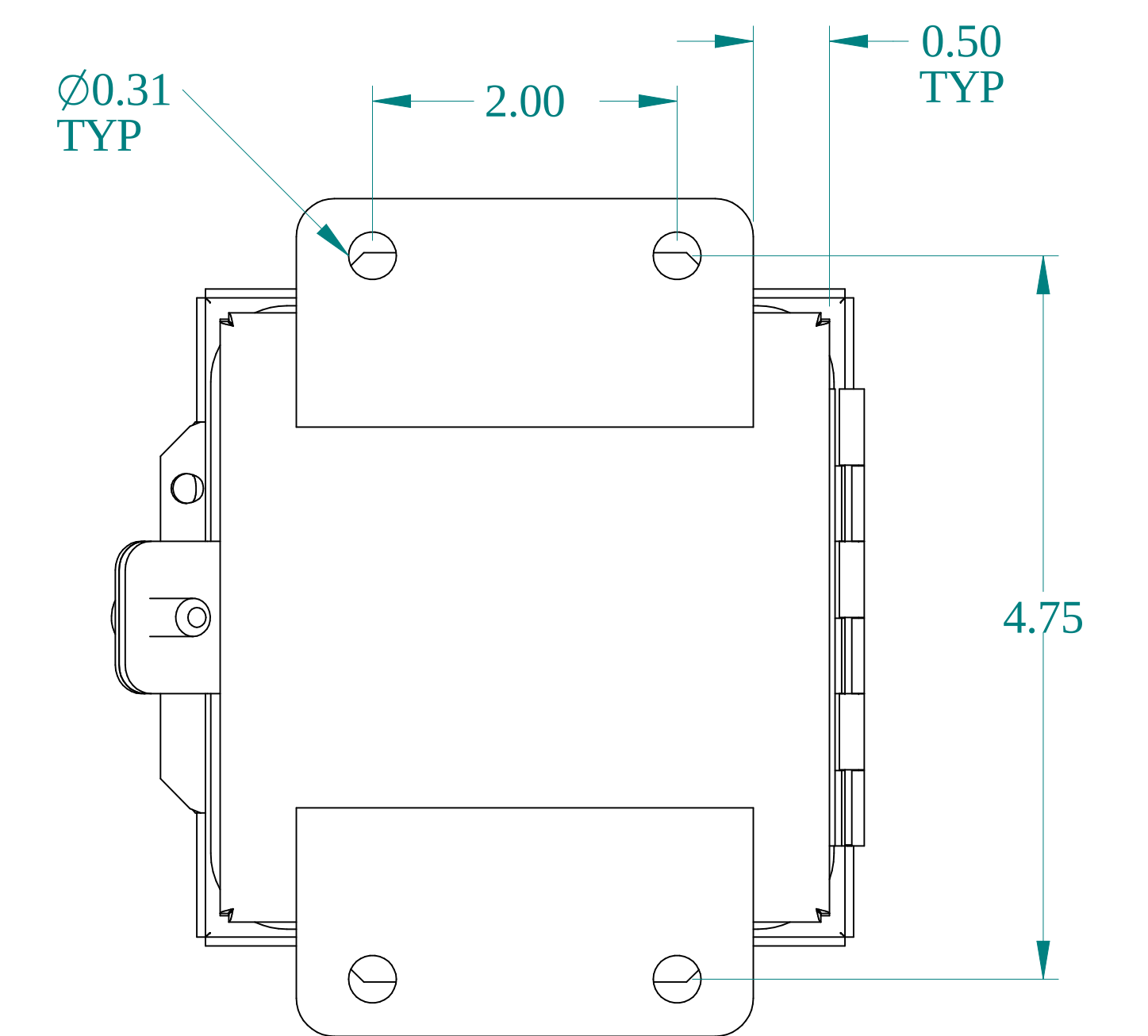
BACK VIEW
