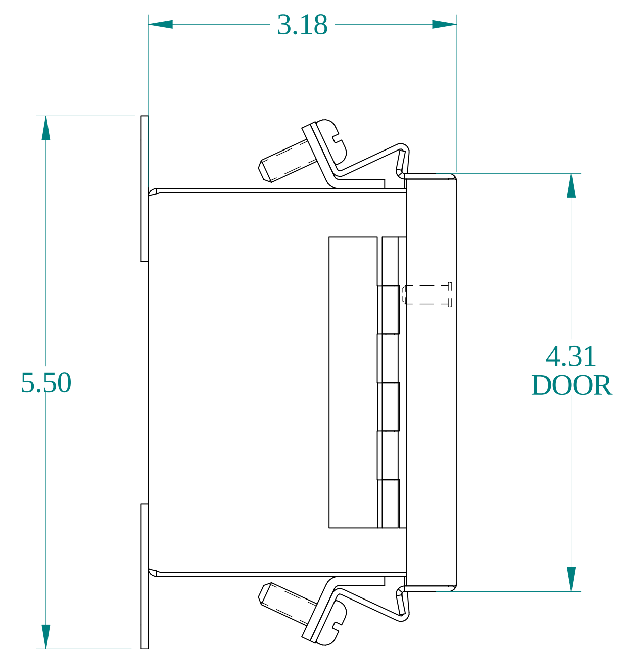
SIDE VIEW
