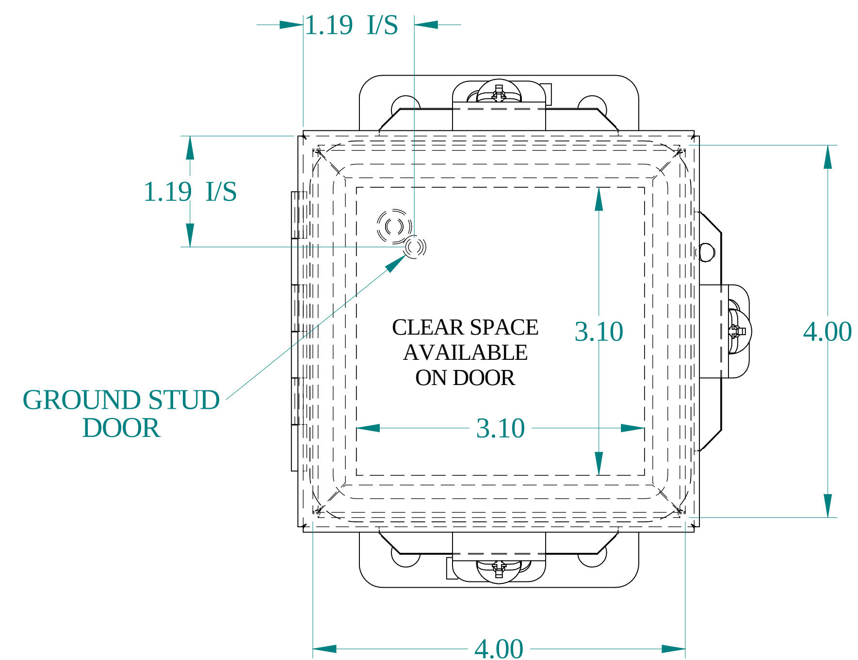
FRONT VIEW
