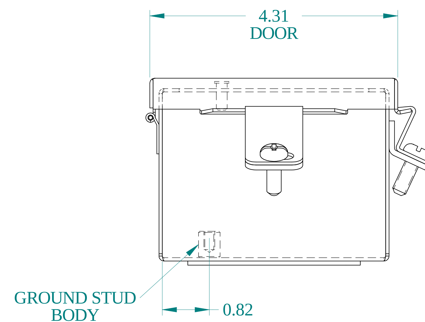
BOTTOM VIEW
