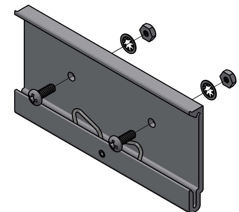
EXPLODED DINCLIP W/ HARDWARE
