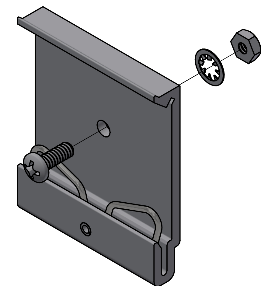
EXPLODED DINCLIP W/ HARDWARE
