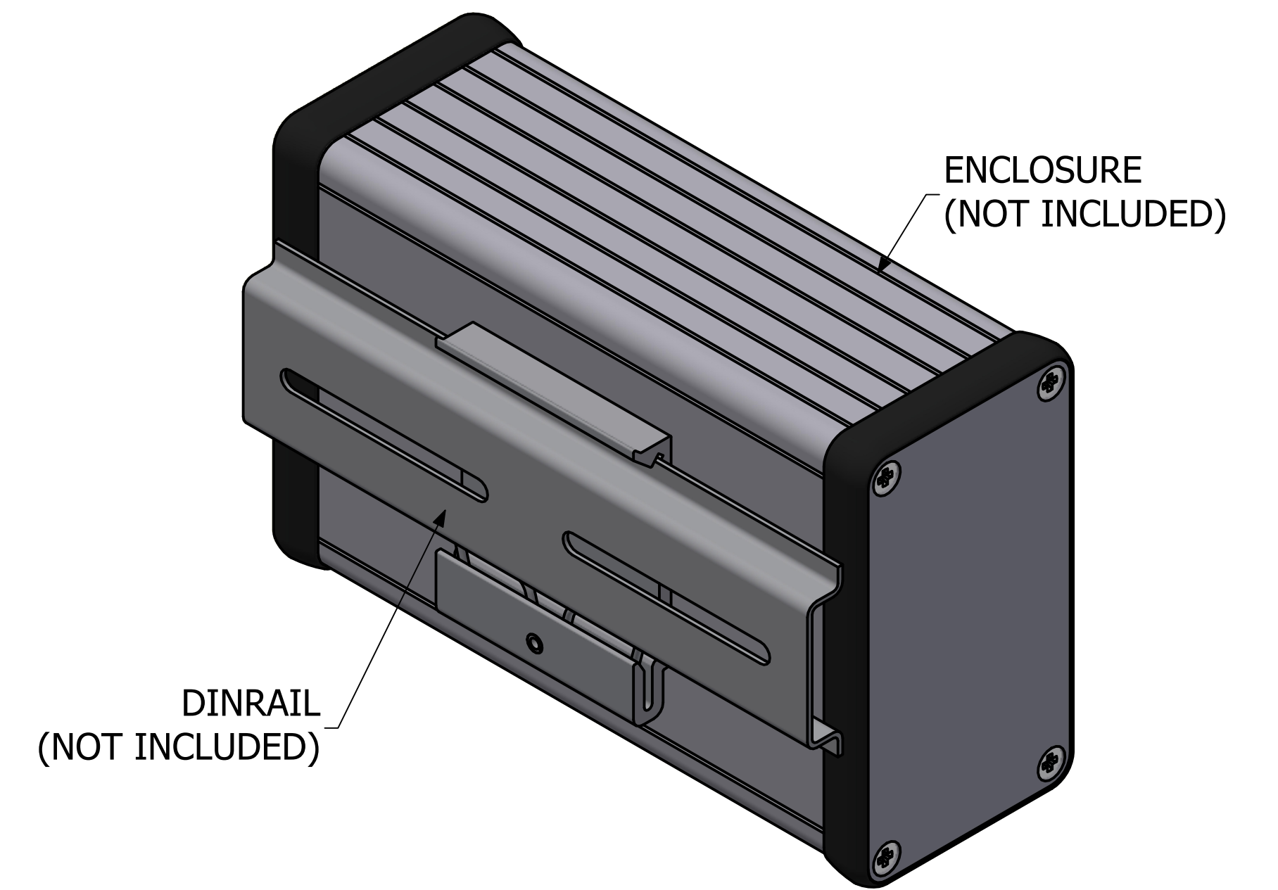
TYPICAL ASSEMBLY
