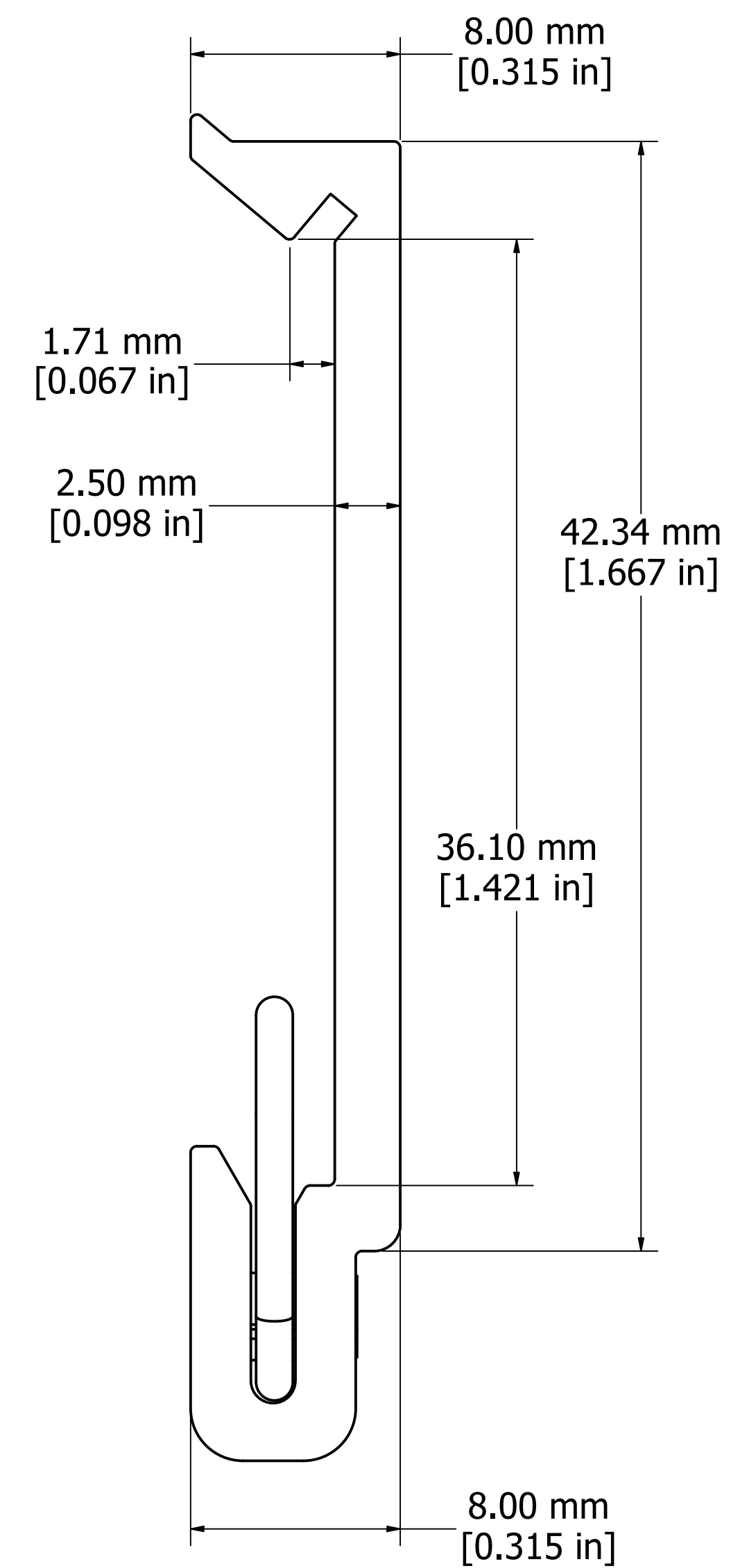
SIDE VIEW
