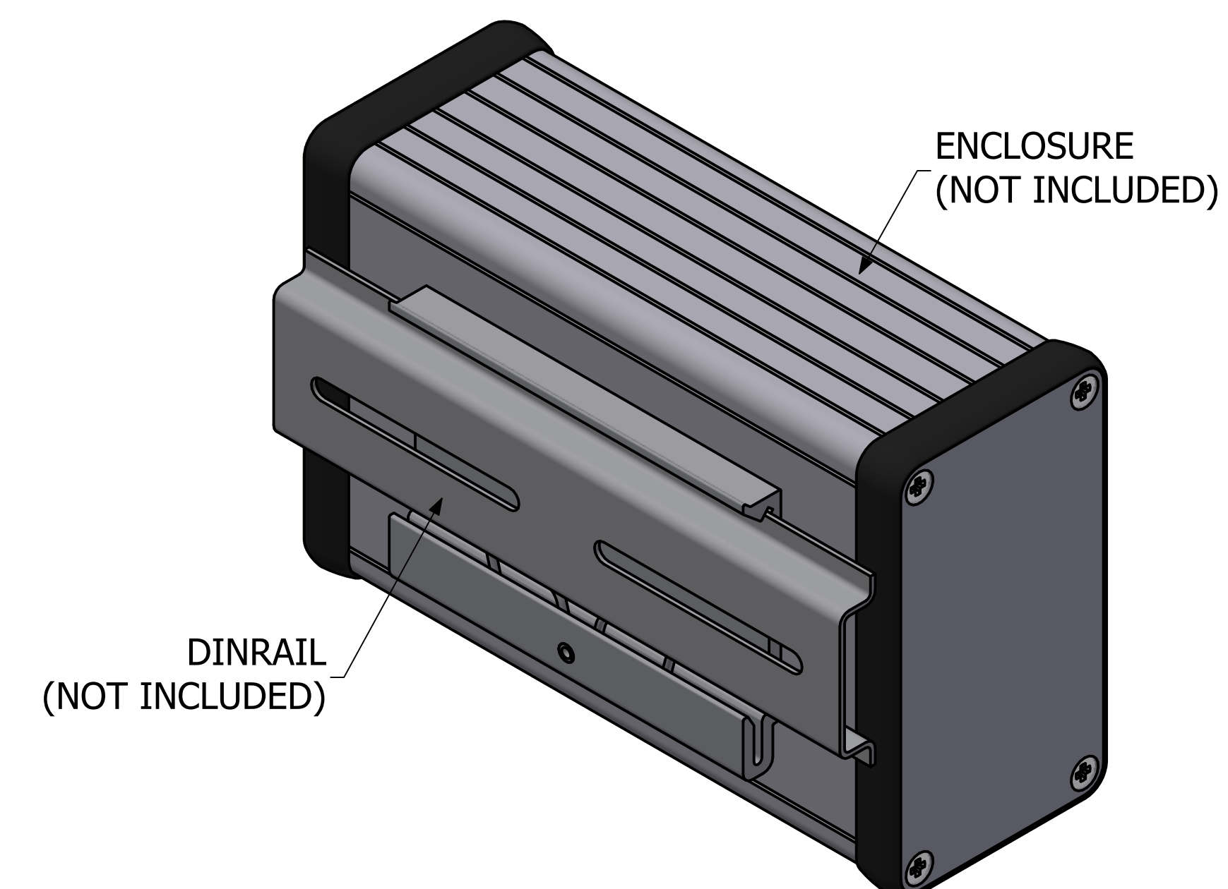
TYPICAL ASSEMBLY
