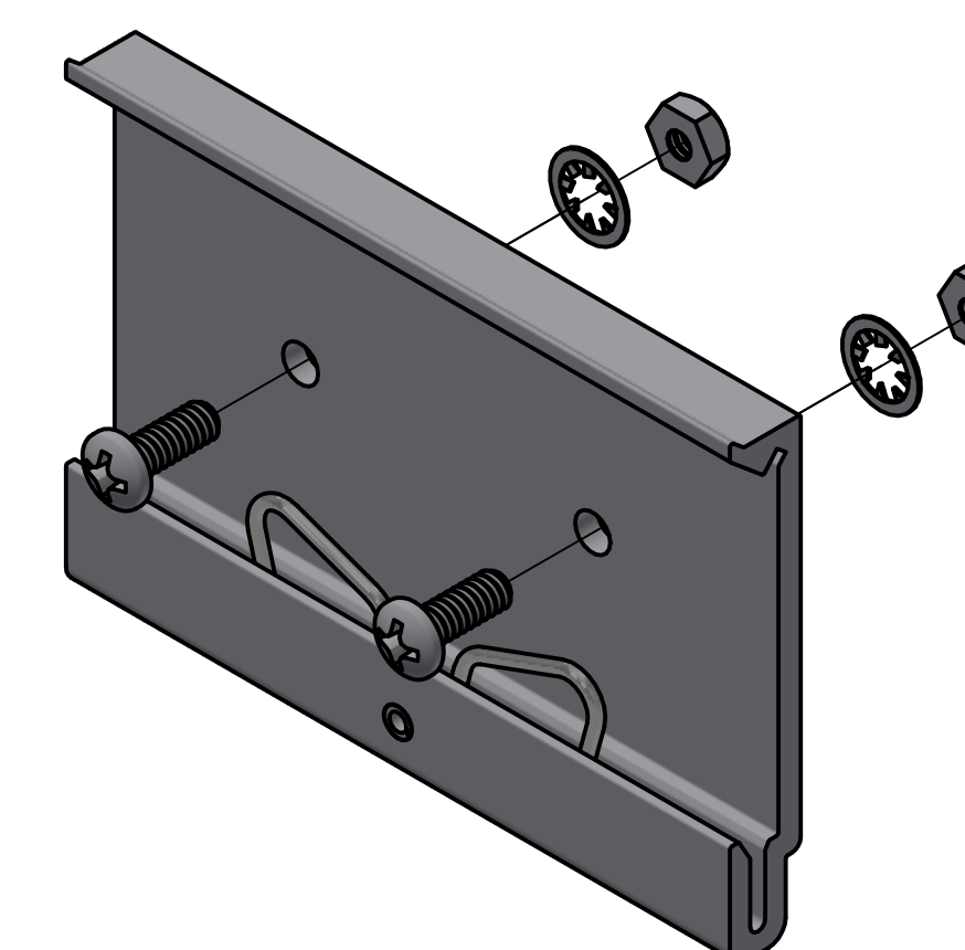
EXPLODED DINCLIP W/ HARDWARE
