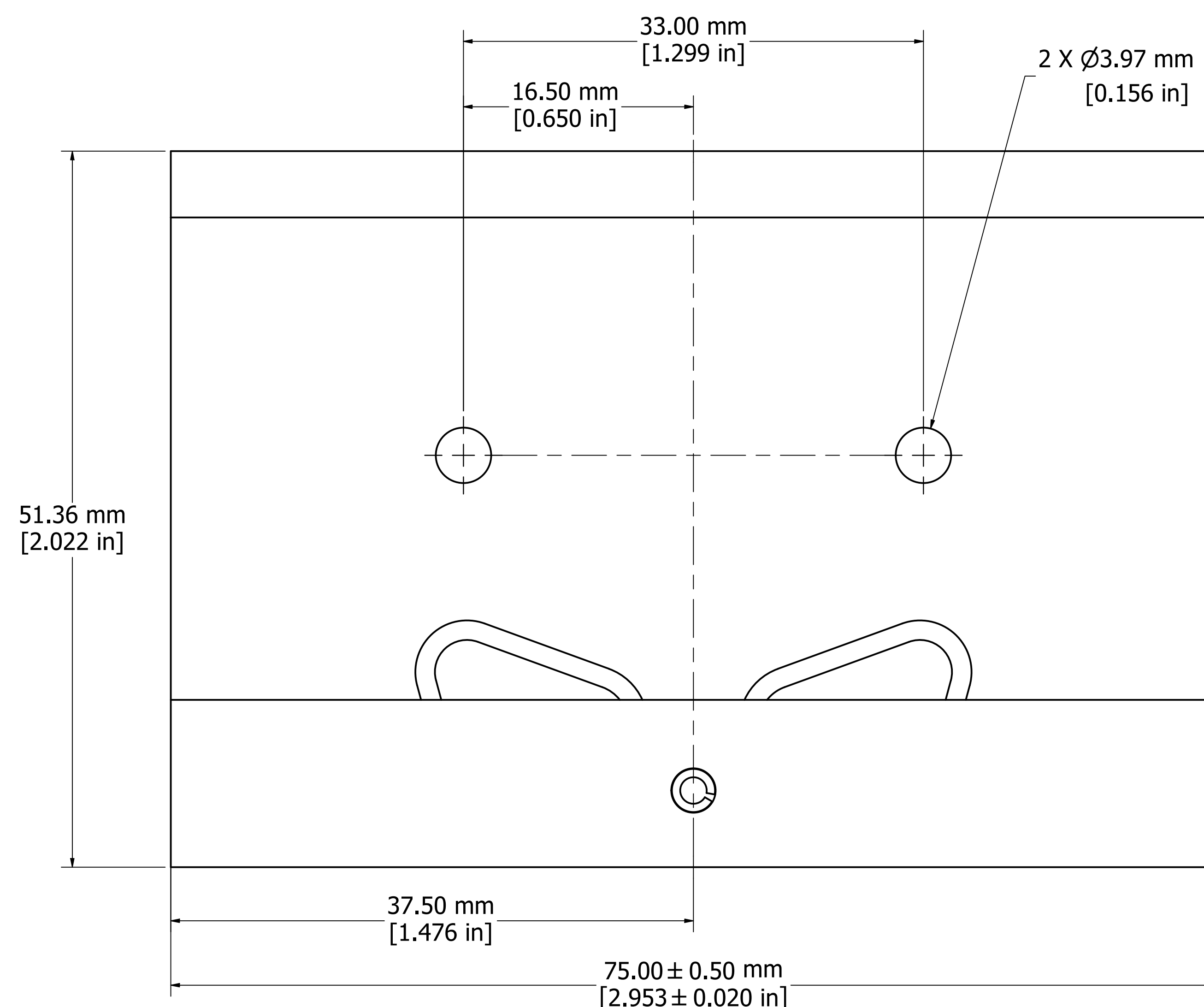
FRONT VIEW
