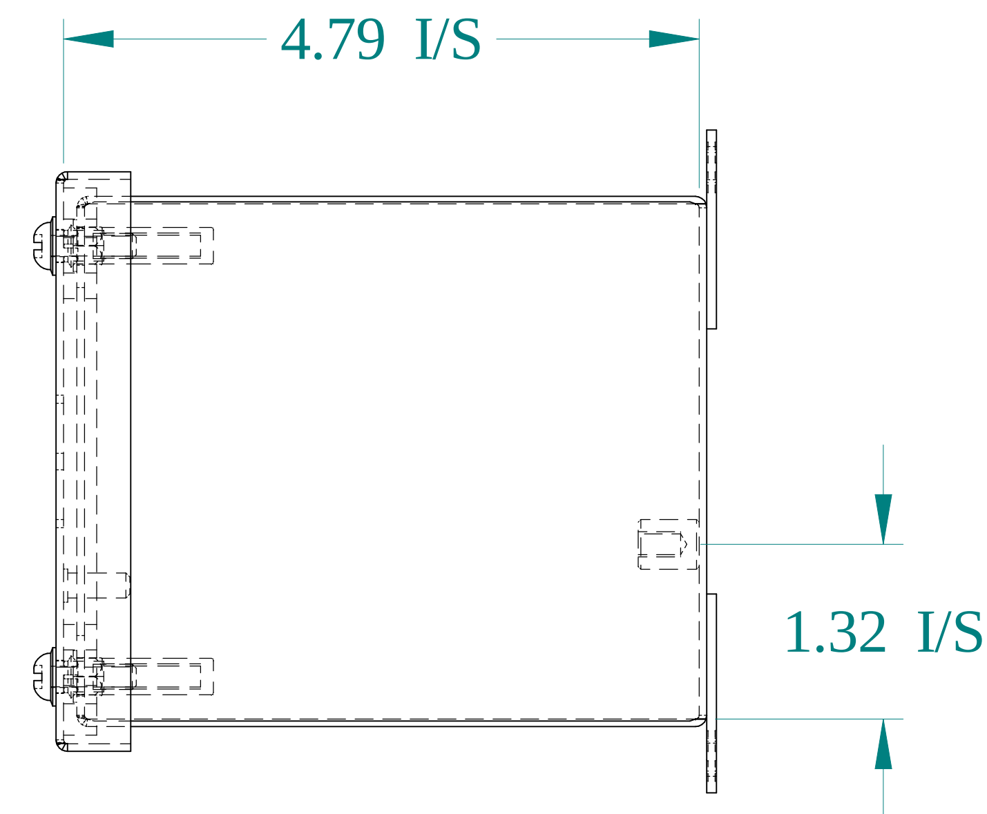
SIDE VIEW
