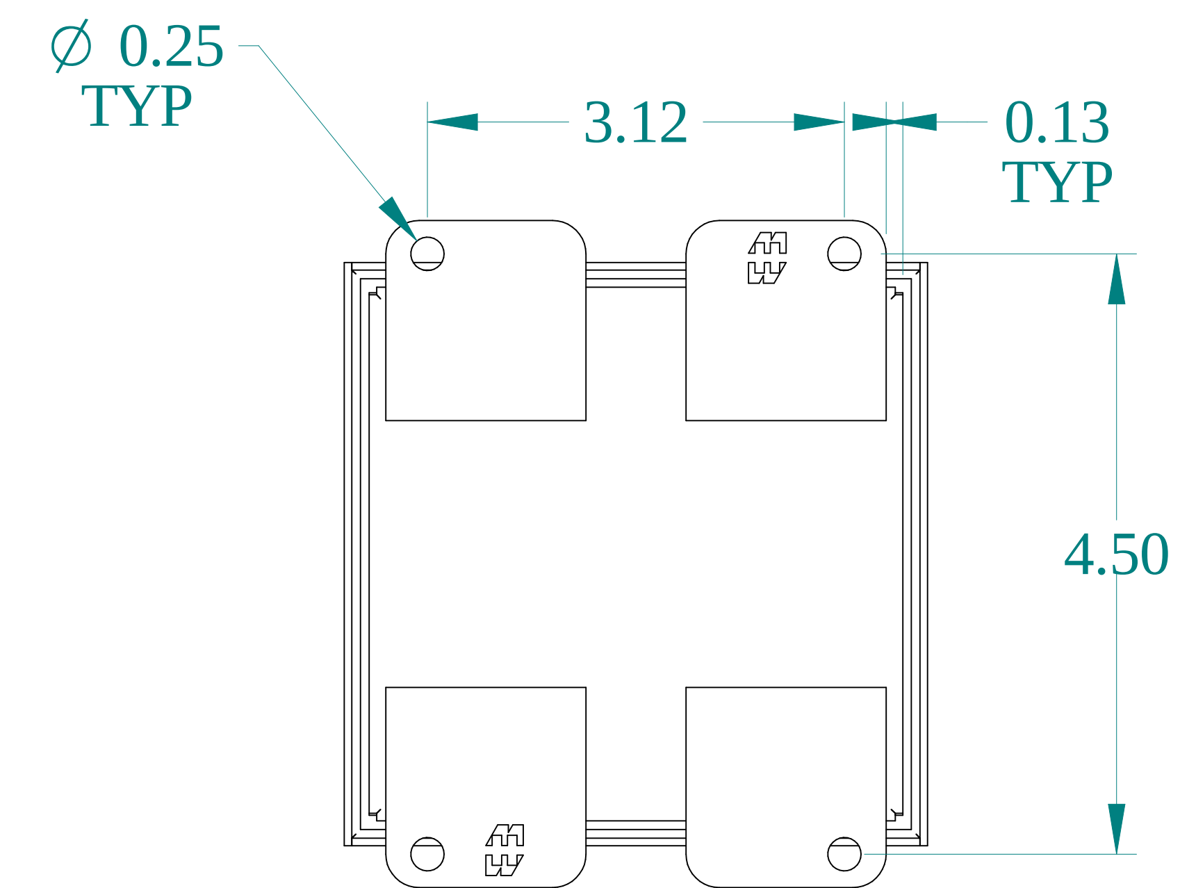
BACK VIEW
