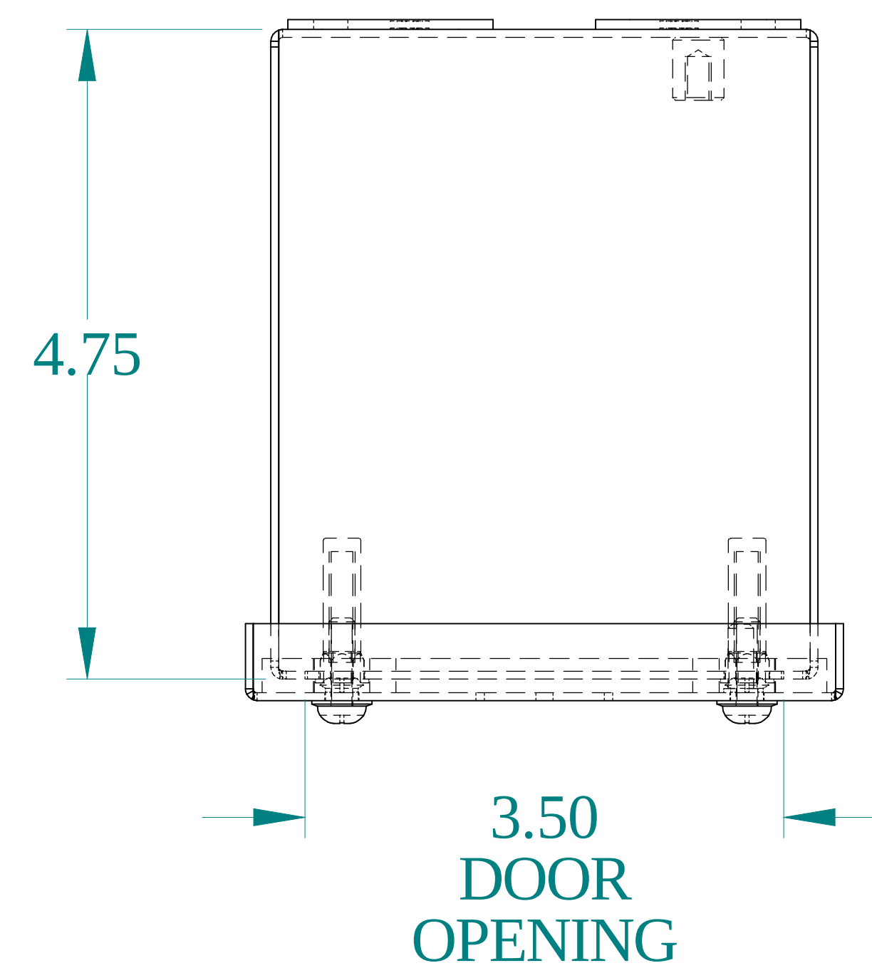
TOP VIEW
