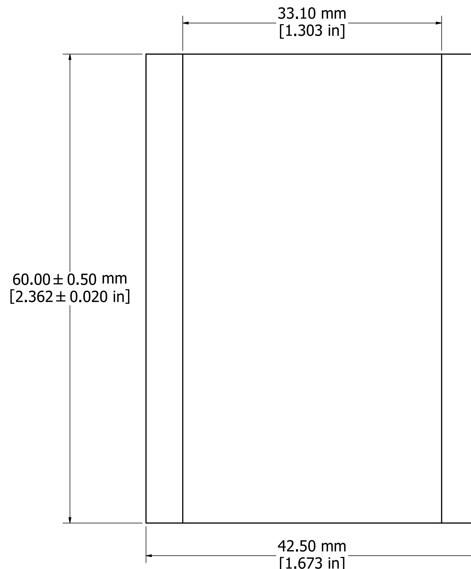
EXTRUSION PROFILE
