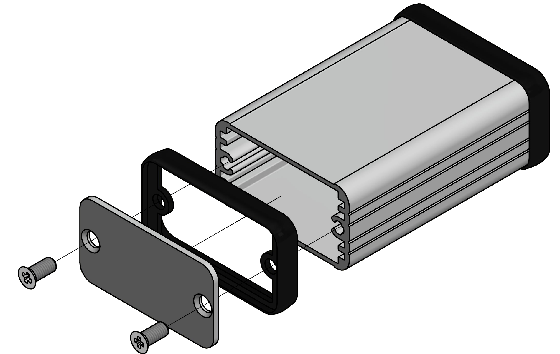
EXPLODED ASSEMBLY VIEW
