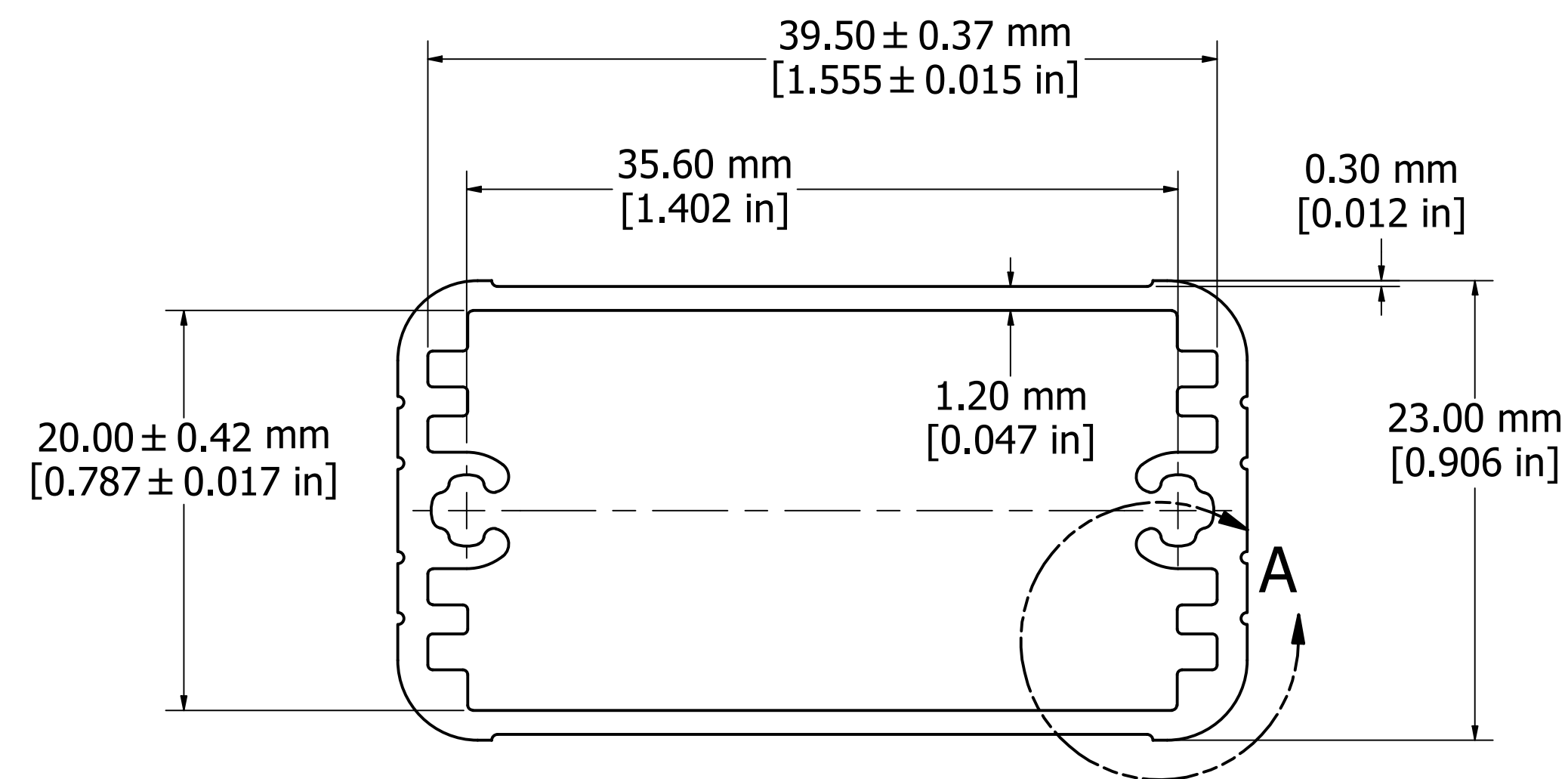
EXTRUSION PROFILE
