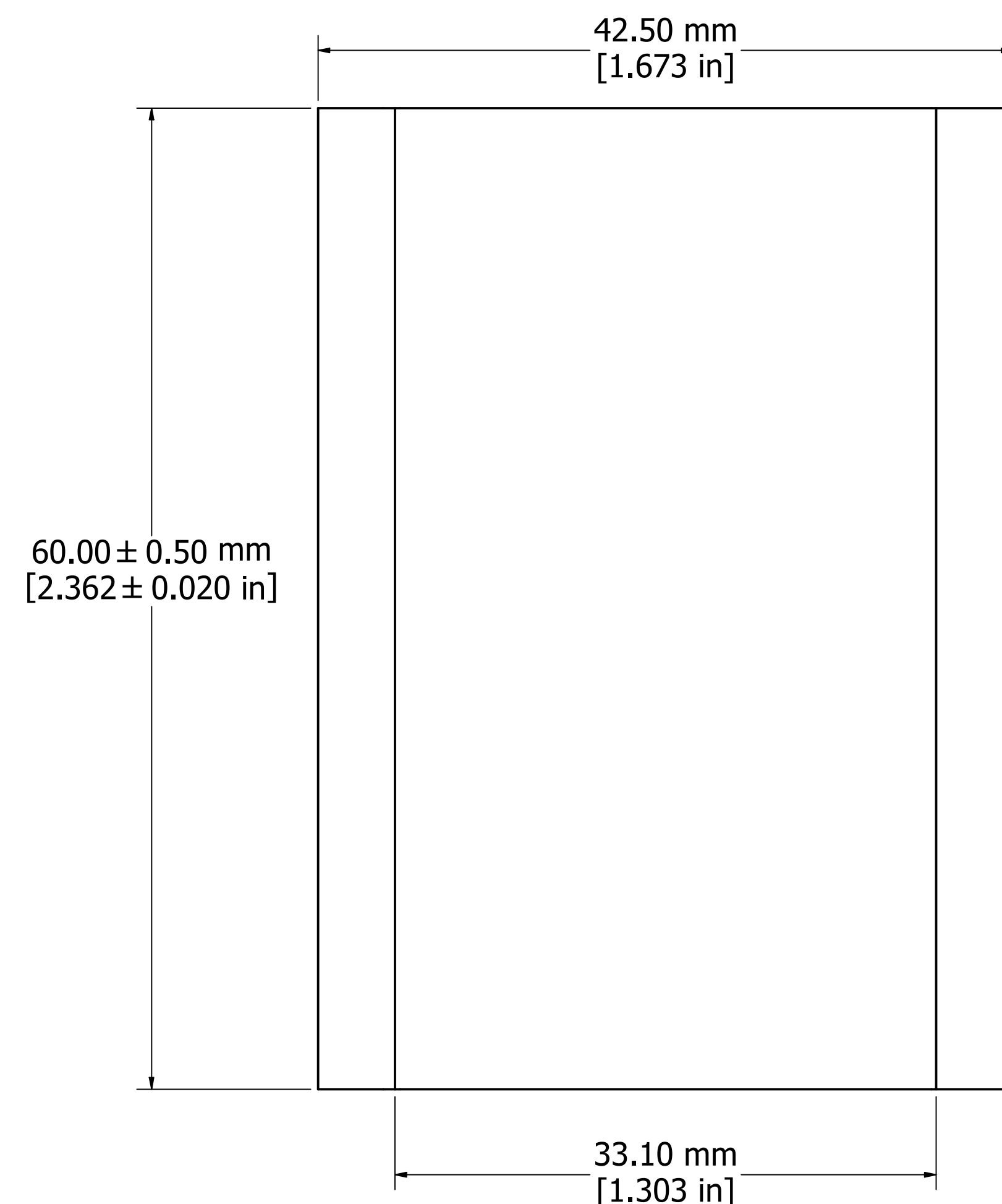
EXTRUSION PROFILE
